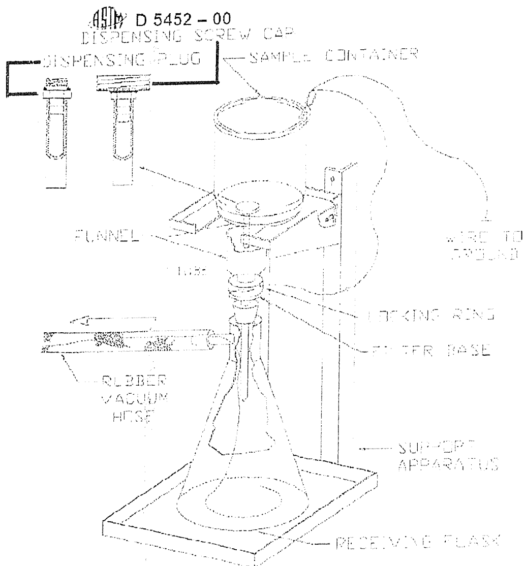
Apparatus for Determining Total Contaminant
